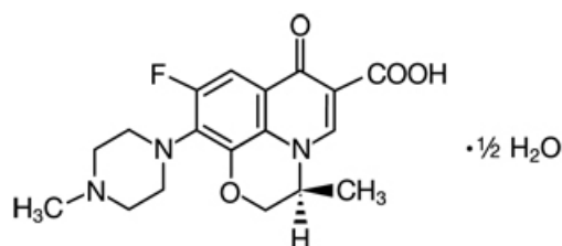
Figure 1: The Chemical Structure of Levofloxacin
