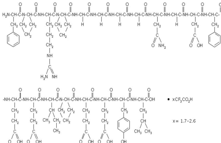
Figure 1: Structure formula for bivalirudin trifluoroacetate
