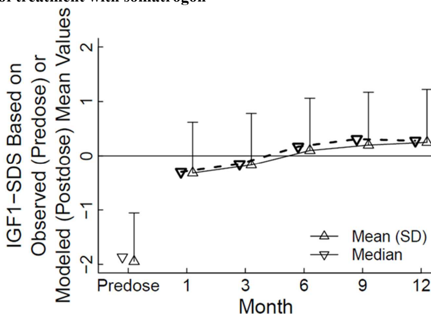
Figure 1. Modeled IGF-1 SDS profiles in pediatric patients with GHD during 12 months of treatment with somatrogon
