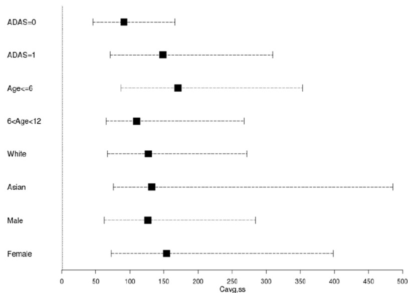
Figure 2. Impact of individual intrinsic factor on somatrogon exposure
